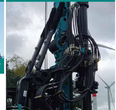
ELECTRICAL SYSTEM: 1. ONE-TOUCH CASING EXTRACTION 2. ONE-TOUCH SOIL THROWING 3. ONE-TOUCH LIFTING 4. ROCK ENTRY MODE 5. ROTATION RESET
