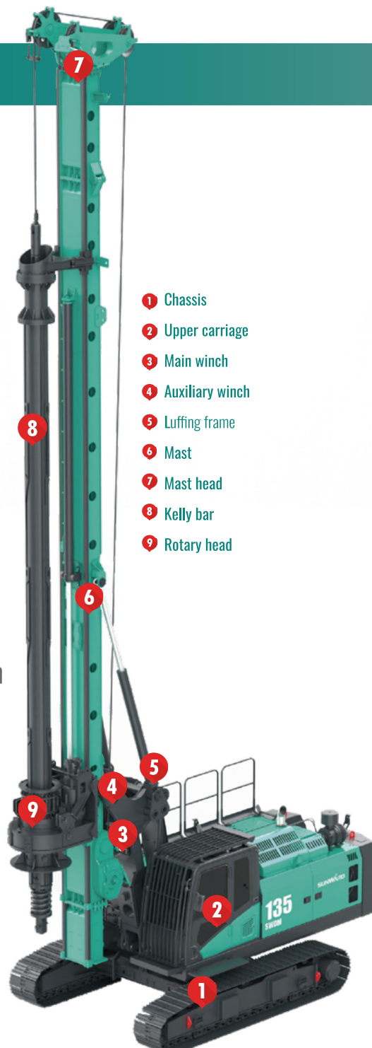
SPACIOUS, QUIET & COMFORTABLE CAB WITH A USER-FRIENDLY CONTROL SYSTEM
